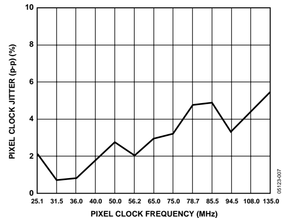
Figure 7. Pixel Clock Jitter vs. Frequency
