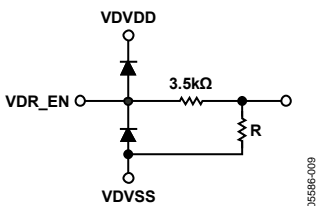
Figure 13. VDR_EN Input
