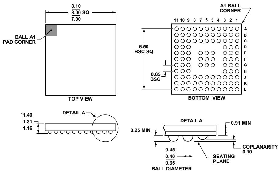
*COMPLIANT TO JEDEC STANDARDS MO-225 WITH THE EXCEPTION TO PACKAGE HEIGHT. Figure 89. 105-Lead Chip Scale Package Ball Grid Array [CSP_BGA] (BC-105) Dimensions shown in millimeters
