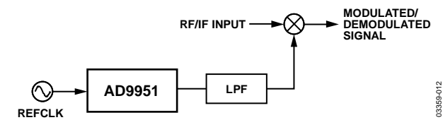
Figure 25. Synchronized LO for Upconversion/Downconversion
