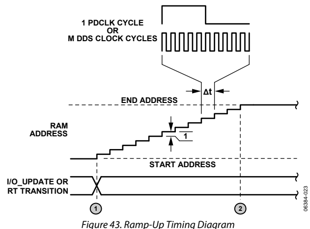
Figure 43. Ramp-Up Timing Diagram
