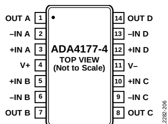
Figure 7. ADA4177-4 14-Lead TSSOP Pin Configuration
