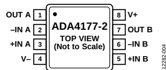
Figure 5. ADA4177-2 8-Lead MSOP Pin Configuration
