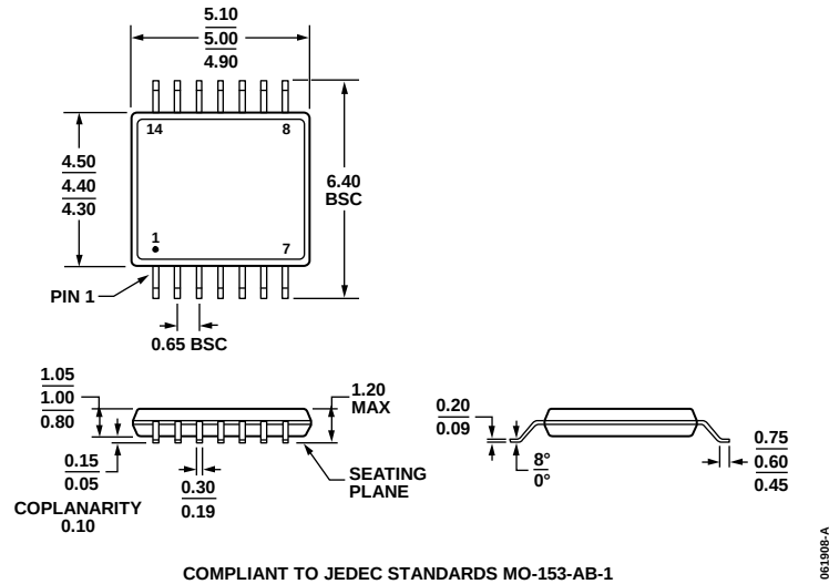
Figure 102. 14-Lead Thin Shrink Small Outline Package [TSSOP] (RU-14) Dimensions shown in millimeters
