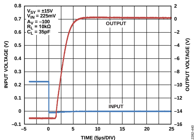
Figure 55. Negative Overload Recovery, V_{SY} = \pm 15V
