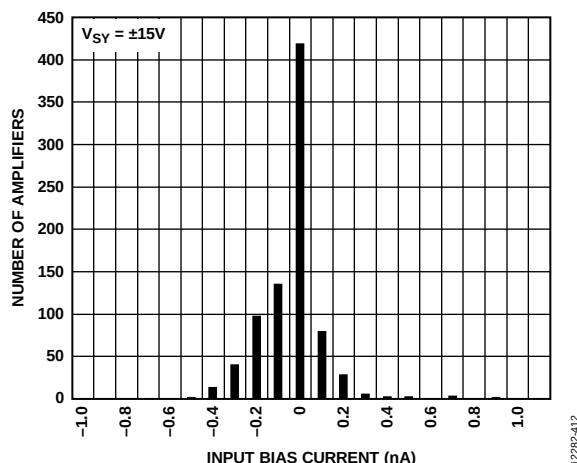
Figure 31. Input Bias Current Distribution, V_{SY} = \pm 15V
