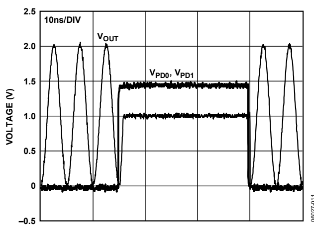
Figure 18. Power-Down Turn On/Turn Off
