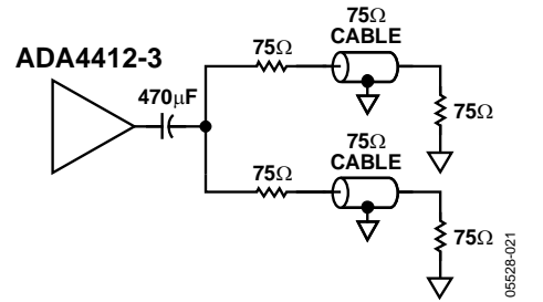
Figure 19. Driving Two AC-Coupled Loads with One Common Coupling Capacitor
