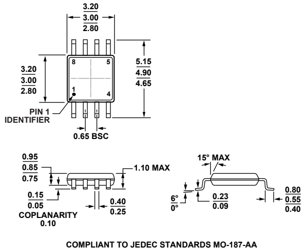
COMPLIANT TO JEDEC STANDARDS MO-187-AA Figure 68. 8-Lead Mini Small Outline Package [MSOP] (RM-8) Dimensions shown in millimeters
