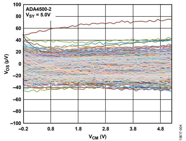
Figure 10. Input Offset Voltage (V OS ) vs. Common-Mode Voltage (V CM ), V SY = 5.0 V
