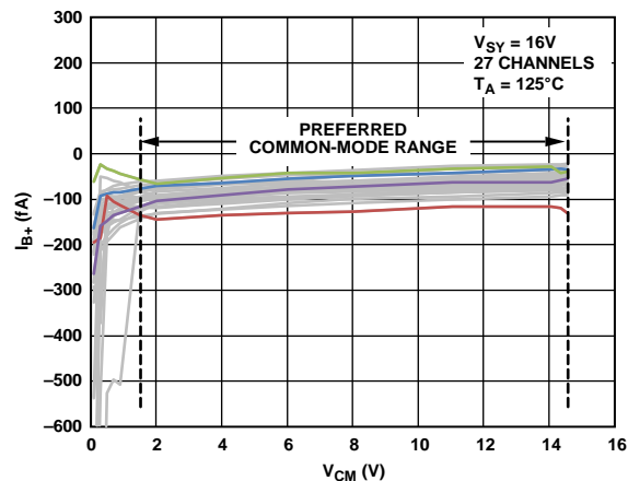
Figure 33. Noninverting Input Bias Current ( I_{B+} ) vs. Common-Mode Voltage ( V_{CM} ), V_{SY} = 16\text{ V} , T_A = 125^\circ\text{C}
