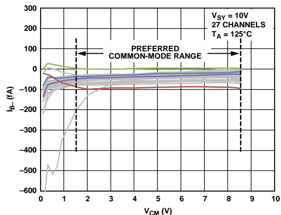
Figure 29. Inverting Input Bias Current ( I_{B-} ) vs. Common-Mode Voltage ( V_{CM} ), V_{SY} = 10\text{ V} , T_A = 125^\circ\text{C}
