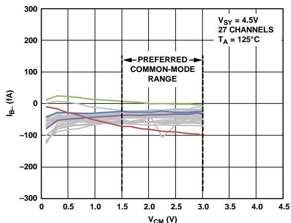
Figure 28. Inverting Input Bias Current ( I_{B-} ) vs. Common-Mode Voltage ( V_{CM} ), V_{SY} = 4.5\text{ V} , T_A = 125^\circ\text{C}
