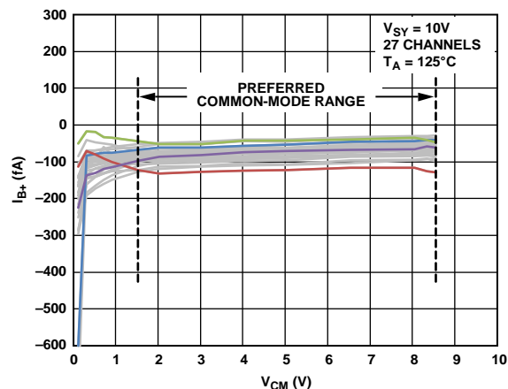
Figure 32. Noninverting Input Bias Current ( I_{B+} ) vs. Common-Mode Voltage ( V_{CM} ), V_{SY} = 10\text{ V} , T_A = 125^\circ\text{C}
