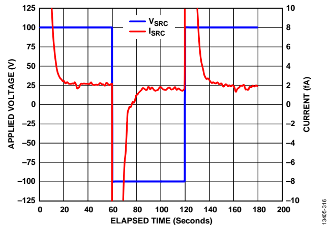
Figure 111. Rogers 4350B Dielectric Relaxation Performance
