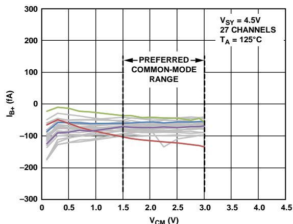
Figure 31. Noninverting Input Bias Current ( I_{B+} ) vs. Common-Mode Voltage ( V_{CM} ), V_{SY} = 4.5\text{ V} , T_A = 125^\circ\text{C}
