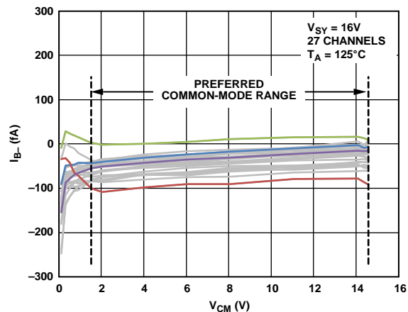
Figure 30. Inverting Input Bias Current ( I_{B-} ) vs. Common-Mode Voltage ( V_{CM} ), V_{SY} = 16\text{ V} , T_A = 125^\circ\text{C}
