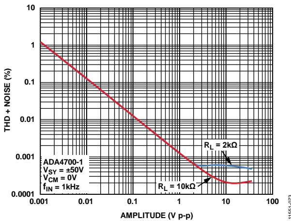
Figure 33. Total Harmonic Distortion + Noise (THD + Noise) vs. Amplitude, V_{SY} = \pm 50V
