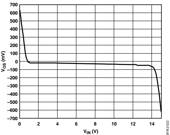
Figure 19. Output Offset Voltage vs. Input Voltage
