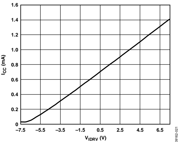
Figure 18. I_{CC} vs. Voltage on IDR Pin ( V_{IDRV} )
