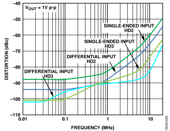
Figure 28. Harmonic Distortion Vs Frequency
