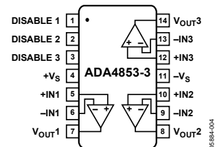
Figure 4. 14-Lead TSSOP
