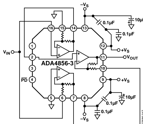
Figure 40. Gain of +5
