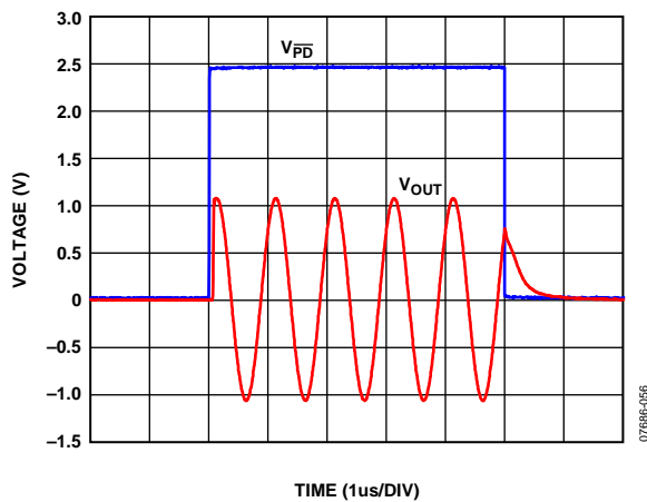
Figure 25. Turn-On/Turn-Off Time
