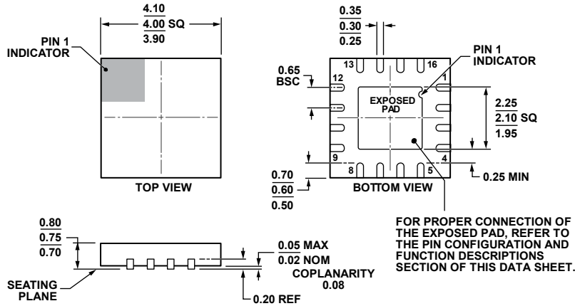
Figure 60. 16-Lead Lead Frame Chip Scale Package [LFCSP] 4 mm × 4 mm Body and 0.75 mm Package Height (CP-16-23) Dimensions shown in millimeters
