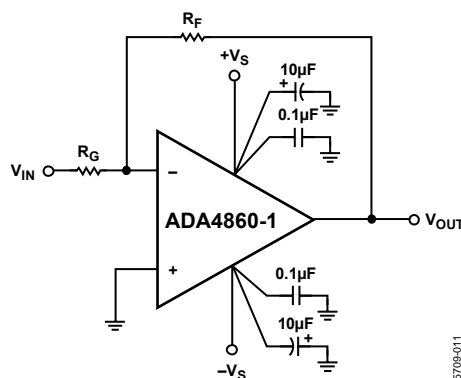
Figure 52. Inverting Gain
