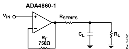
Figure 53. Driving Capacitive Loads
