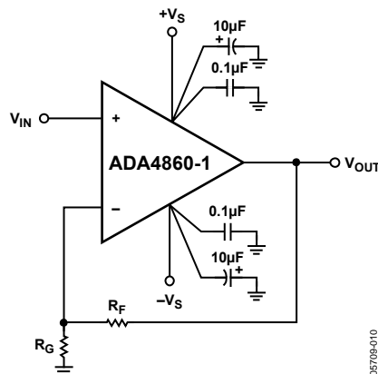
Figure 51. Noninverting Gain
