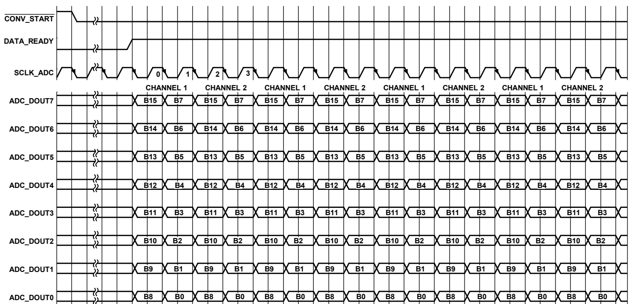
Figure 45. PPI, 2-Channel
