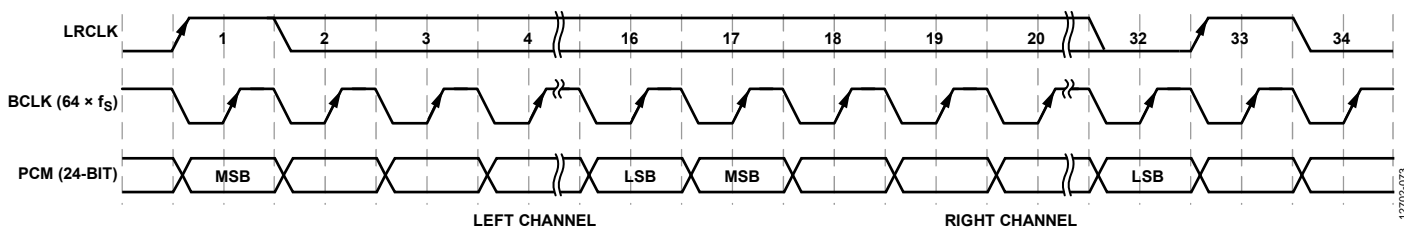
Figure 72. PCM/DSP Mode, 16 Bits per Channel, Long Frame Sync
