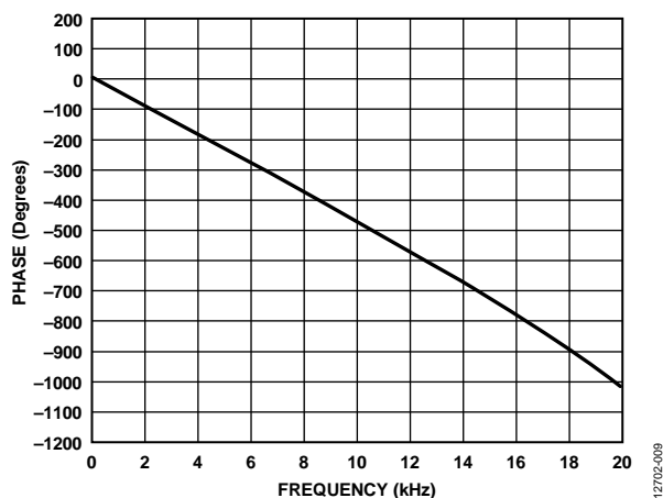
Figure 9. Phase vs. Frequency, 20 kHz Bandwidth, f_s = 48 kHz, Signal Path = AIN0 to ASRC to ADC_SDAT00
