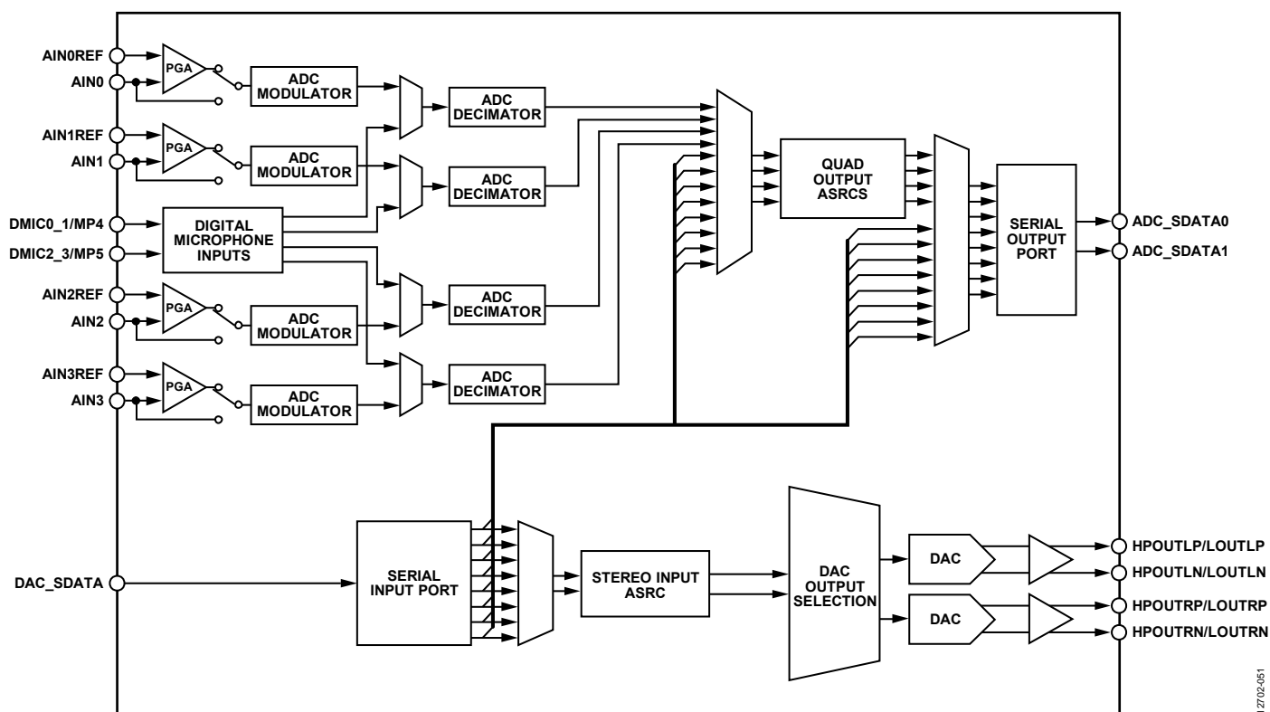
Figure 50. Input and Output Signal Routing
