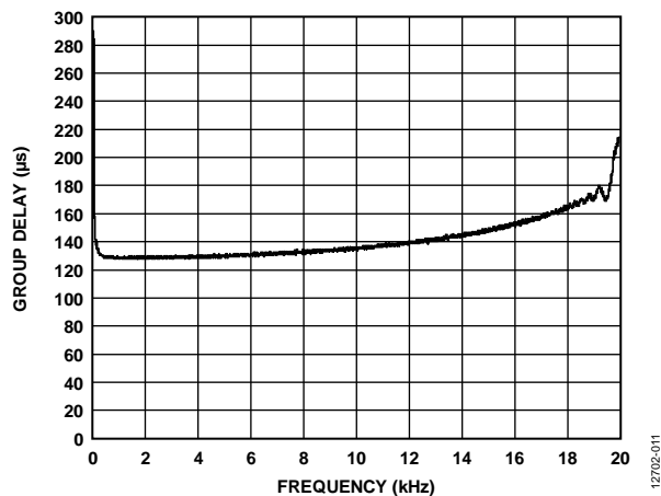
Figure 11. Group Delay vs. Frequency, f_s = 48 kHz, Signal Path = AIN0 to ASRC to ADC_SDAT00
