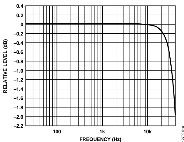
Figure 10. Relative Level vs. Frequency, f_s = 96 kHz, Signal Path = AIN0 to ASRC to ADC_SDAT00
