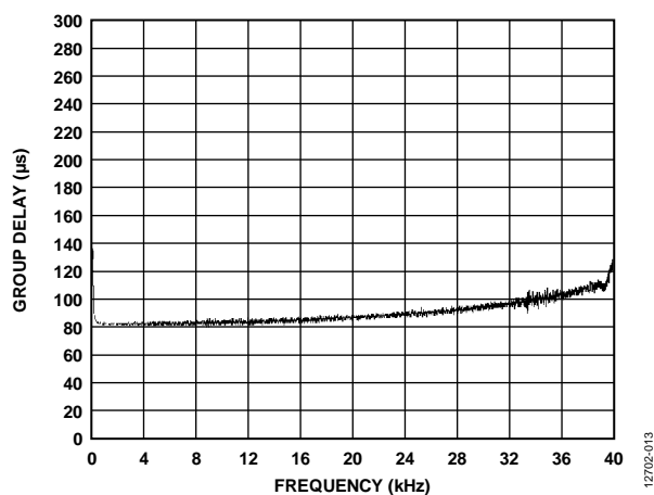
Figure 13. Group Delay vs. Frequency, f_s = 96 kHz, Signal Path = AIN0 to ASRC to ADC_SDAT00
