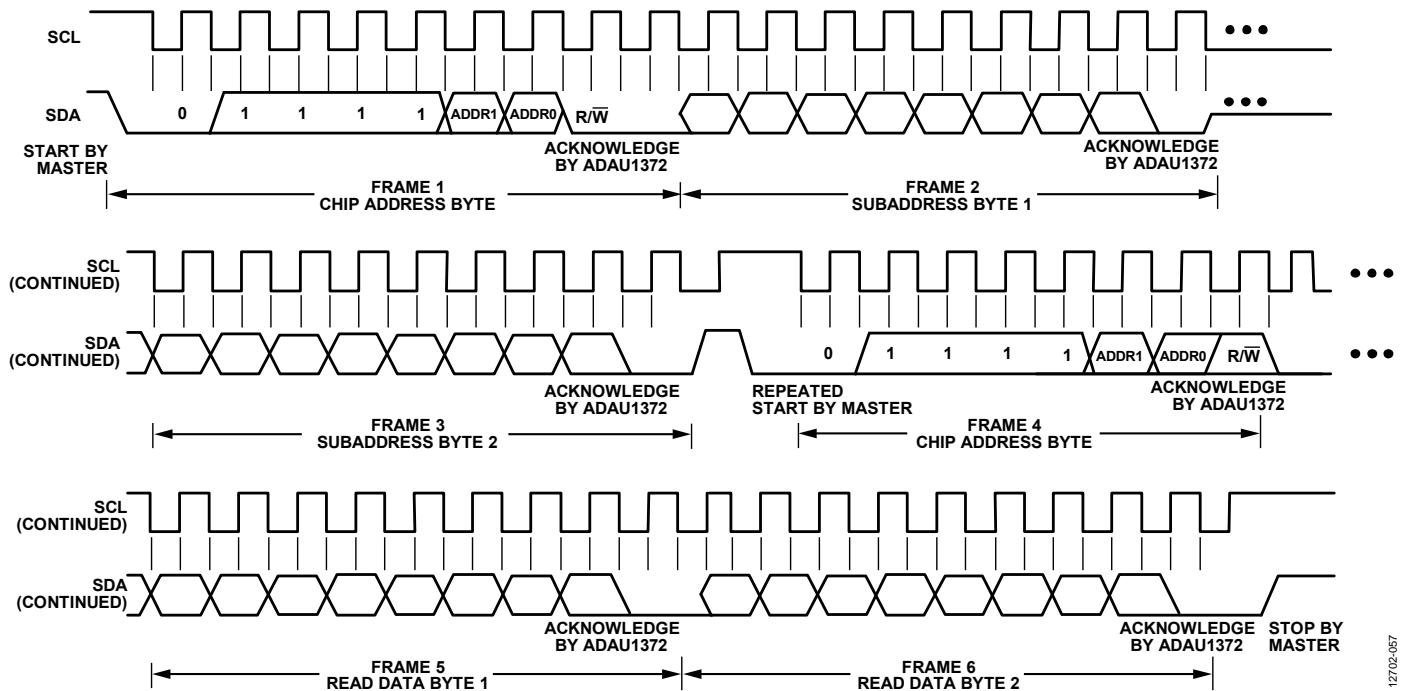
Figure 56. I²C Read from the ADAU1372 Clocking and Data Format
