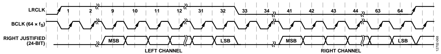
Figure 67. Right Justified Mode, 24 Bits per Channel
