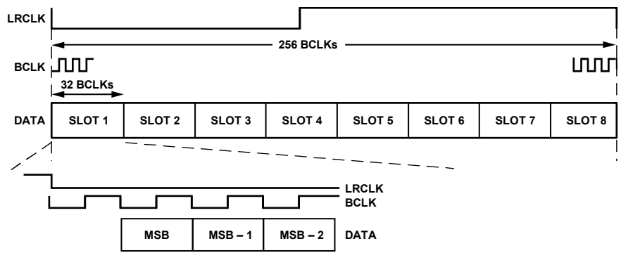
Figure 69. 8-Channel TDM Mode
