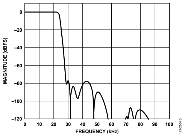
Figure 46. Total Interpolation Response, f_s = 96 kHz
