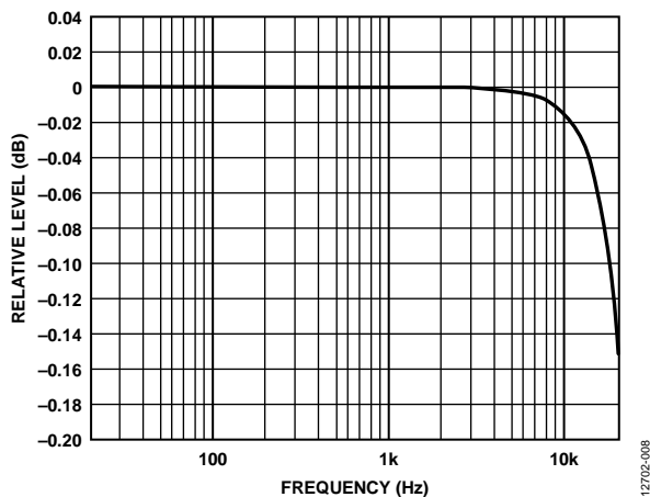
Figure 8. Relative Level vs. Frequency, f_s = 48 kHz, Signal Path = AIN0 to ASRC to ADC_SDAT00
