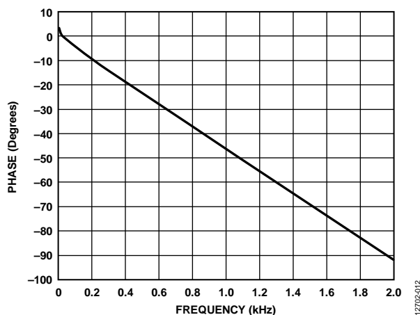
Figure 12. Phase vs. Frequency, 2 kHz Bandwidth, f_s = 48 kHz, Signal Path = AIN0 to ASRC to ADC_SDAT00
