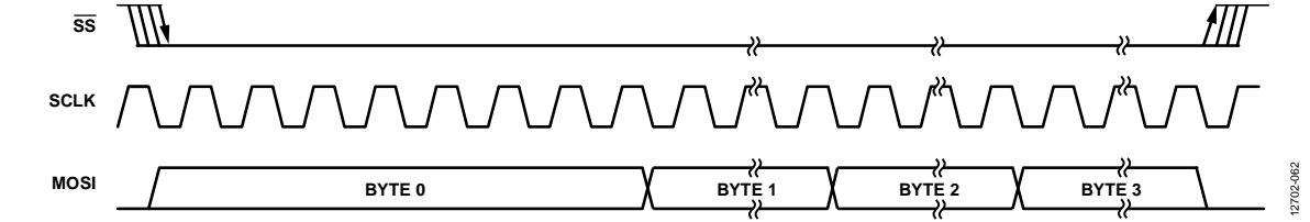
Figure 61. SPI Write to the ADAU1372 Clocking and Data Format (Burst Write Mode)
