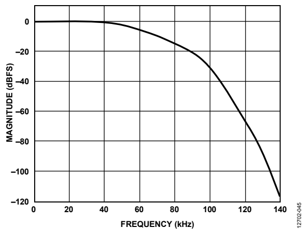
Figure 45. Total Decimation Response, f_s = 192 kHz, Serial Port f_s = 192 kHz
