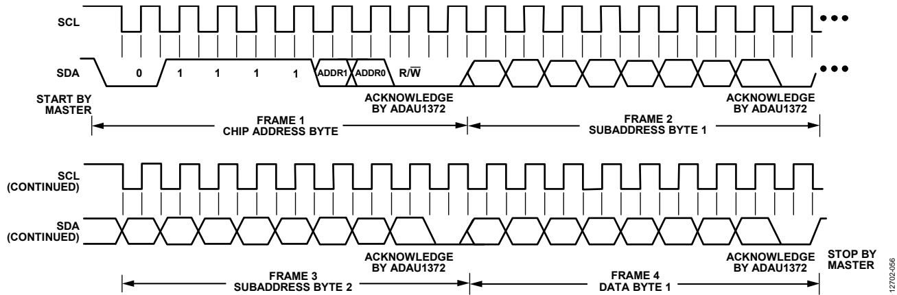
Figure 55. I²C Write to the ADAU1372 Clocking and Data Format
