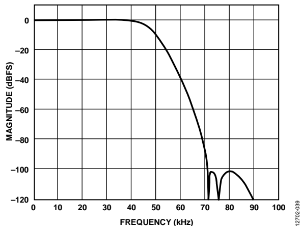
Figure 39. Total Decimation Response, f_s = 96 kHz, Serial Port f_s = 96 kHz
