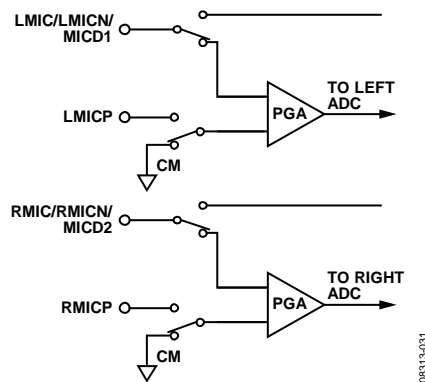
Figure 33. Single-Ended Input Configuration
