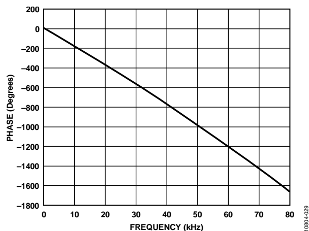
Figure 30. Phase vs. Frequency, 80 kHz Bandwidth, f_s = 192 kHz, Signal Path = AIN0 to ASRC to ADC_SDATA0
