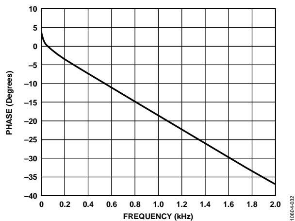
Figure 33. Phase vs. Frequency, 2 kHz Bandwidth, f_s = 192 kHz, Signal Path = AIN0 to ASRC to ADC_SDATA0
