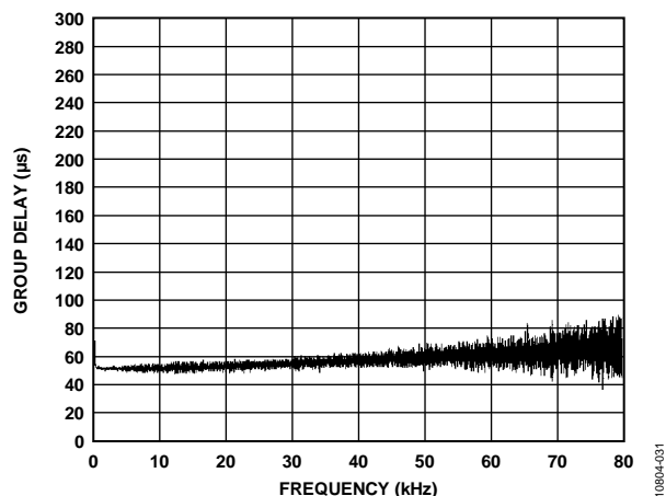
Figure 32. Group Delay vs. Frequency, f_s = 192 kHz, Signal Path = AIN0 to ASRC to ADC_SDATA0
