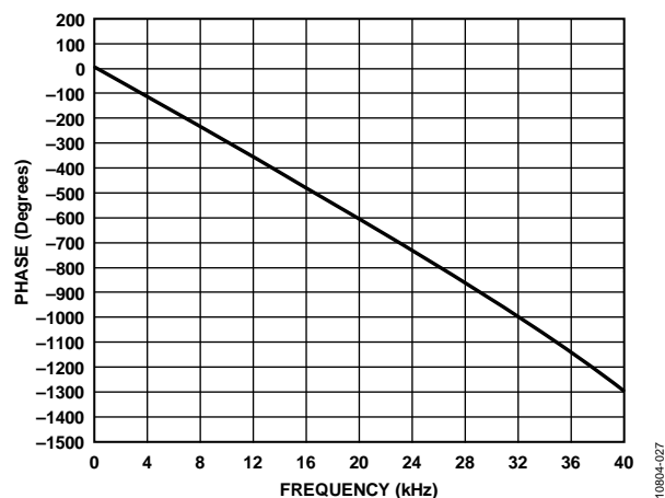
Figure 28. Phase vs. Frequency, 40 kHz Bandwidth, f_s = 96 kHz, Signal Path = AIN0 to ASRC to ADC_SDATA0
