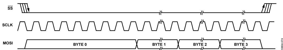
Figure 89. SPI Write to ADAU1772 Clcking (Single-Write Mode)
