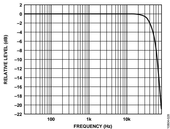
Figure 29. Relative Level vs. Frequency, f_s = 192 kHz, Signal Path = AIN0 to ASRC to ADC_SDATA0
