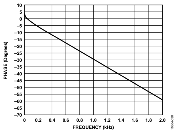
Figure 31. Phase vs. Frequency, 2 kHz Bandwidth, f_s = 96 kHz, Signal Path = AIN0 to ASRC to ADC_SDATA0
