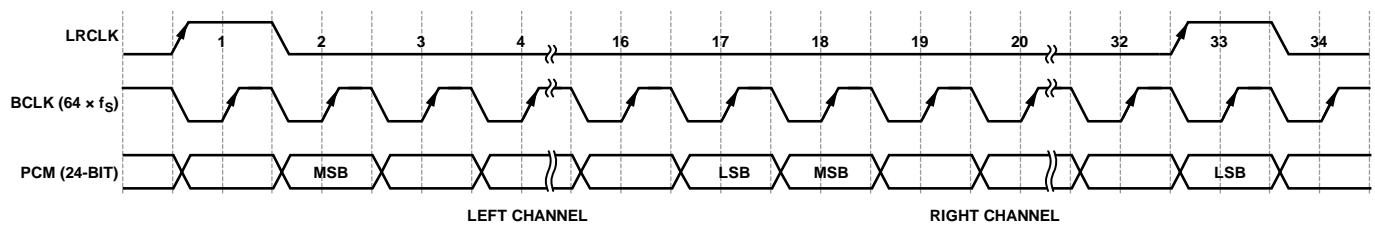
Figure 100. PCM/DSP Mode, 16 Bits per Channel, Short Frame Sync
