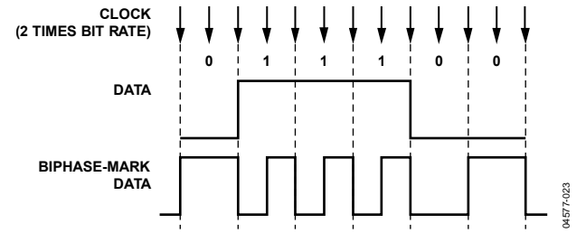
Figure 43. Biphase-Mark Encoding
