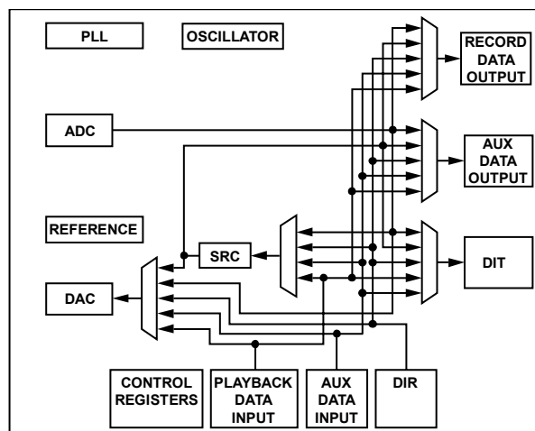
Figure 52. Datapath
