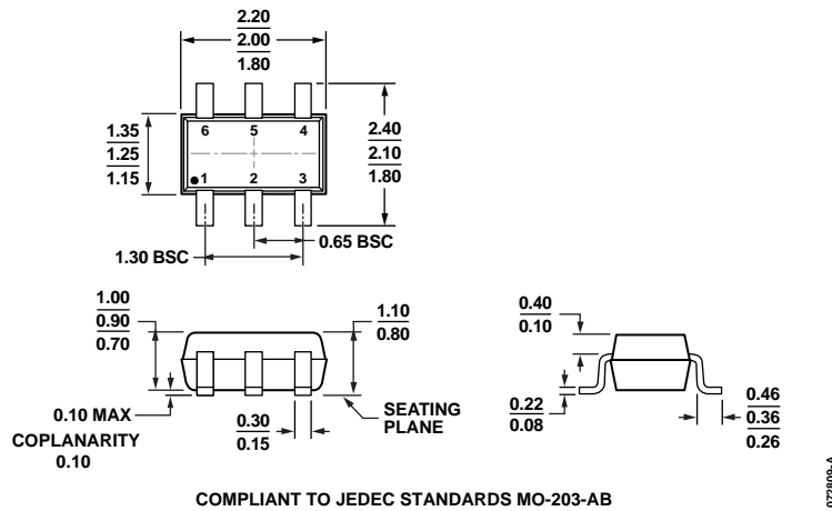
Figure 26. 6-Lead Thin Shrink Small Outline Transistor Package [SC70] (KS-6)
