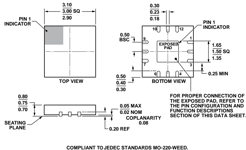
Figure 27. 12-Lead Lead Frame Chip Scale Package [LFCSP] 3 mm x 3 mm and 0.75 mm Package Height (CP-12-5)
