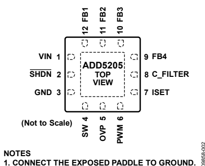
Figure 3. Pin Configuration
