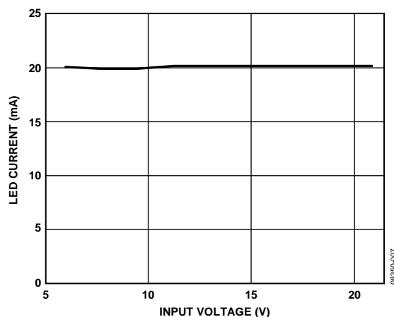
Figure 7. LED Current vs. Input Voltage ( I_{LED} = 20mA )
