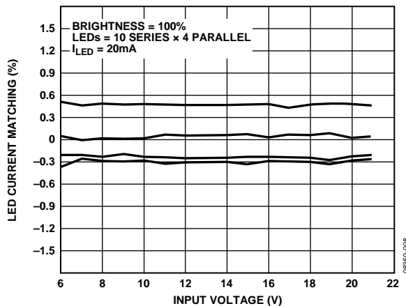
Figure 8. LED Current Matching vs. Input Voltage
