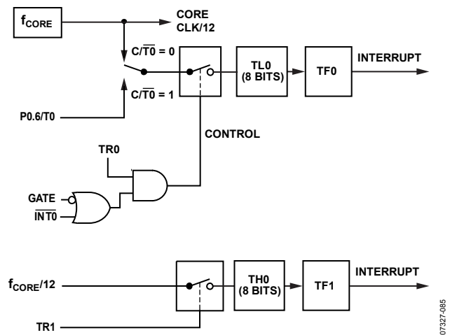
Figure 85. Timer/Counter 0, Mode 3
