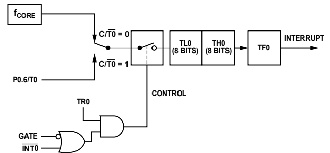
Figure 83. Timer/Counter 0, Mode 1
