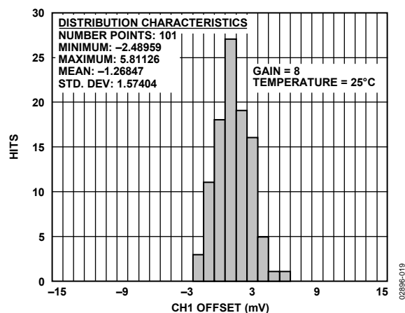
Figure 19. Channel 1 Offset Distribution (Gain = 8)
