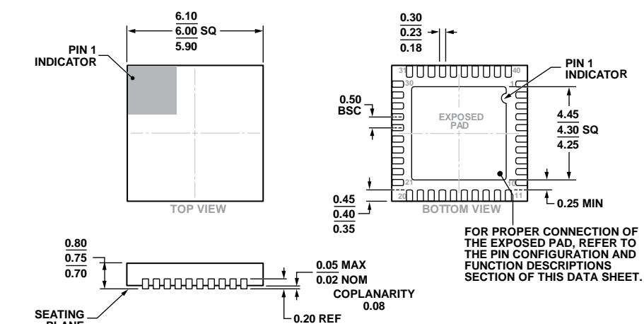
Figure 48. 40-Lead Lead Frame Chip Scale Package [LFCSP_WQ] 6 mm × 6 mm Body, Very Very Thin Quad (CP-40-10) Dimensions shown in millimeters
