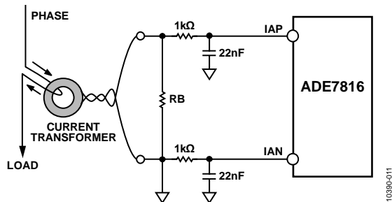
Figure 26. Current Transformer Input Connections
