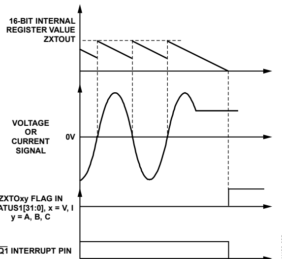
Figure 44. Zero-Crossing Timeout Detection
