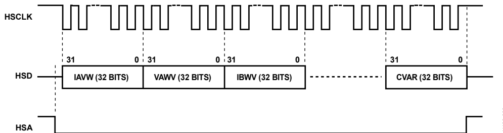
Figure 101. HSDC Communication for HGAP = 0, HXFER[1:0] = 00, and HSAPOL = 0; HSIZE Is Irrelevant
