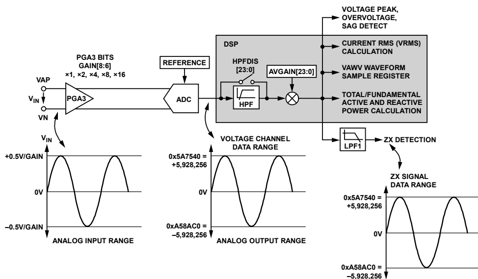
Figure 42. Voltage Channel Datapath
