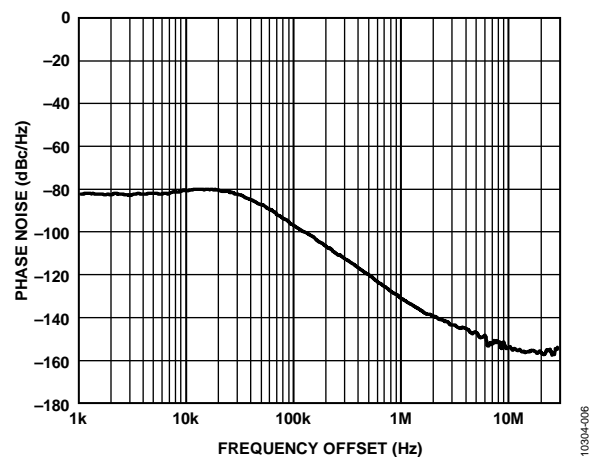
Figure 6. Closed-Loop Phase Noise, RF = 12.5 GHz , PDF = 2.5 MHz , Loop Bandwidth = 20 kHz
