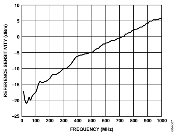
Figure 7. REF_IN Sensitivity
