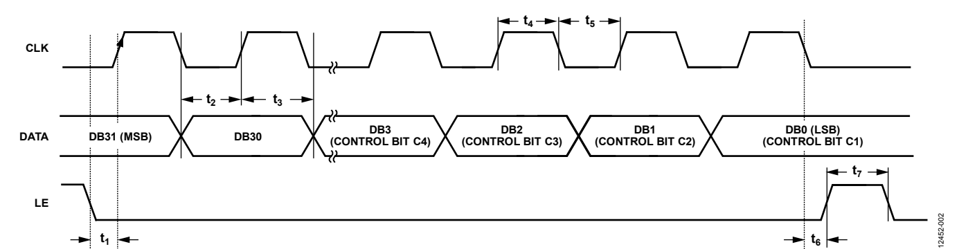
Figure 2. Timing Diagram
