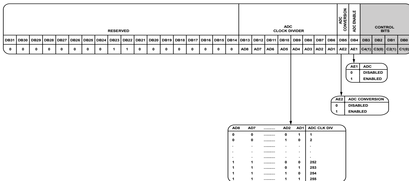
Figure 40. Register 10
