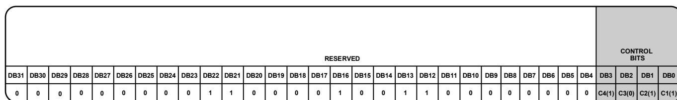
Figure 41. Register 11 (0x0061300B)
