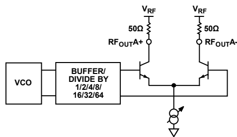
Figure 37. Output Stage
