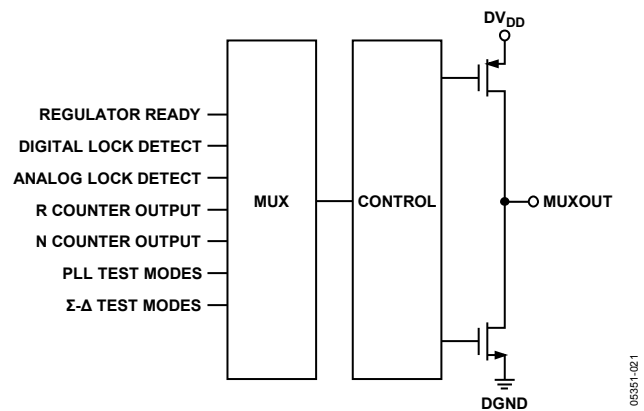
Figure 21. MUXOUT Circuit
