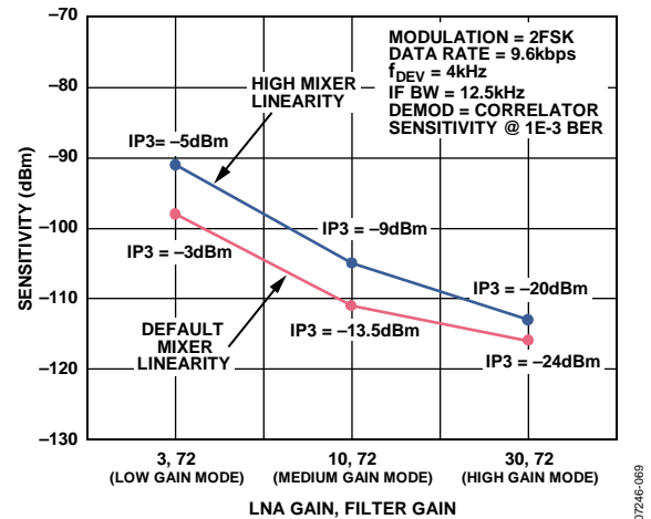
Figure 31. Receive Sensitivity vs. LNA/IF Filter Gain and Mixer Linearity Settings (The input IP3 at each setting is also shown)
