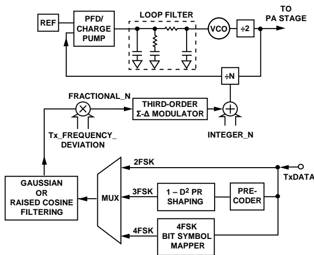
Figure 41. Transmit Modulation Implementation
