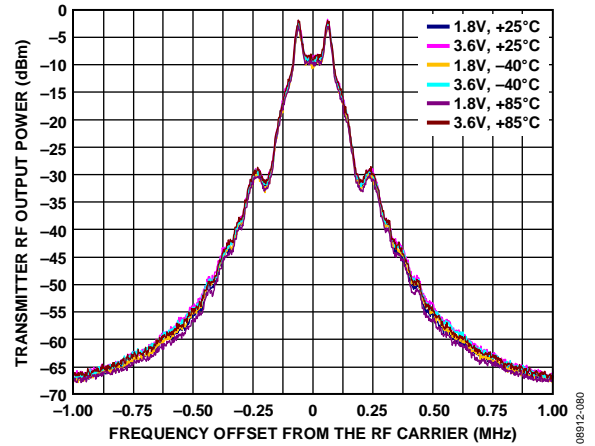
Figure 54. 125 Mbps FSK ( f_{DEV} = \pm 60 kHz) Mode Transmitter Spectrum vs. Temperature and VDD_BAT, f_{CHANNEL} = 2.45 GHz, Output Power = 3 dBm
