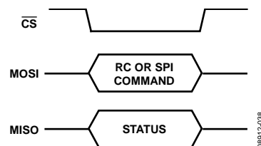
Figure 102. Command Write
