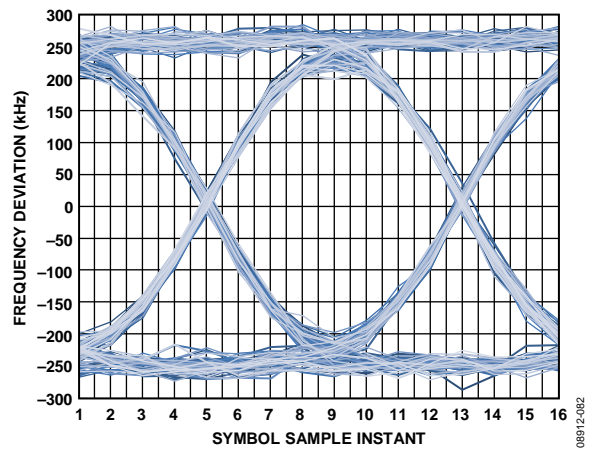
Figure 56. 500 kbps FSK ( f_{DEV} = \pm 250 kHz) Mode Transmitter Eye Diagram, f_{CHANNEL} = 2.45 GHz, Output Power = 3 dBm, VDD_BAT = 3.6 V, Temperature = 25°C
