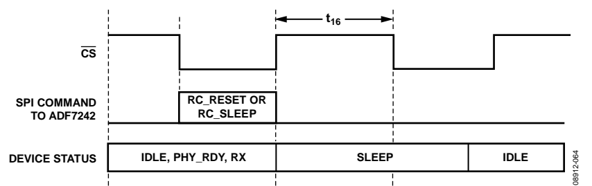
Figure 5. Wake-Up After an \text{RC\_RESET} or \text{RC\_SLEEP} Command
