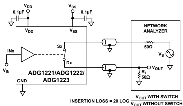
Figure 31. Test Circuit 9—Bandwidth
