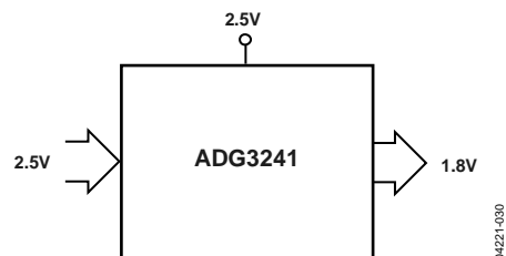
Figure 30. 2.5 V to 1.8 V Voltage Translation, \overline{SEL} = 2.5 V_{CC}
