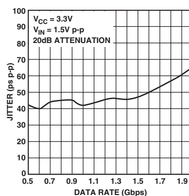
TPC 15. Jitter vs. Data Rate; PRBS 31
