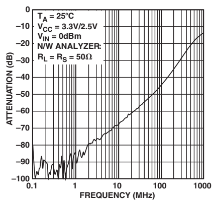
TPC 13. Off Isolation vs. Frequency
