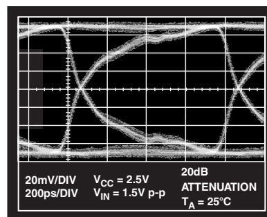
TPC 18. Eye Pattern; 1.244 Gbps, V_{CC} = 2.5 V, PRBS 31
