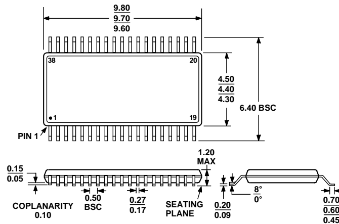
Figure 14. 38-Lead Thin Shrink Small Outline Package [TSSOP] (RU-38)
