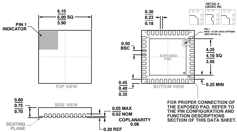
Figure 13. 40-Lead Lead Frame Chip Scale Package [LFCSP] 6 x 6 mm Body and 0.75 mm Package Height (CP-40-9)
