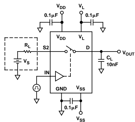
Test Circuit 5. Charge Injection
