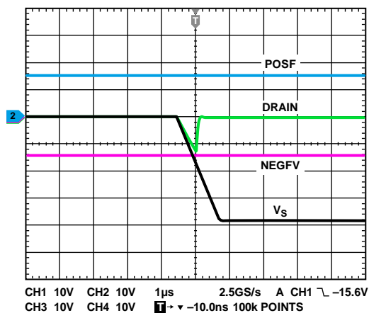
Figure 32. Drain Output Response to Negative Overvoltage
