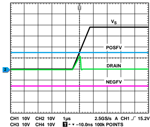
Figure 31. Drain Output Response to Positive Overvoltage
