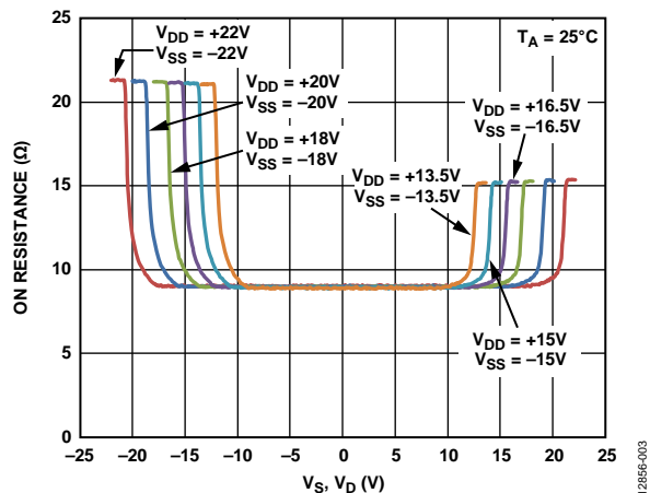
Figure 4. R_{ON} as a Function of V_S and V_D , Dual Supply
