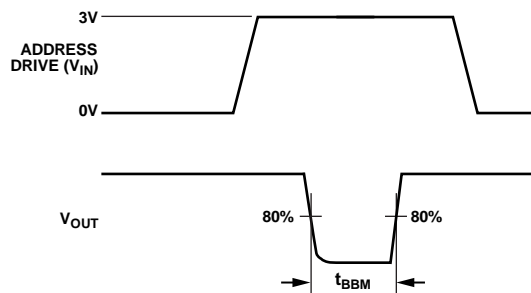
Figure 25. Break-Before-Make Delay, t_{\text{BBM}}
