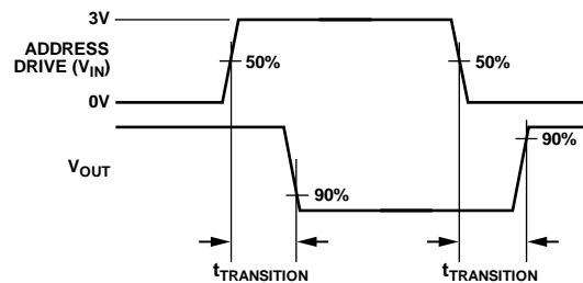
Figure 24. Transition Time, t_{\text{TRANSITION}}
