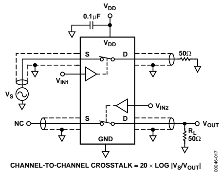
Figure 16. Channel-to-Channel Crosstalk
