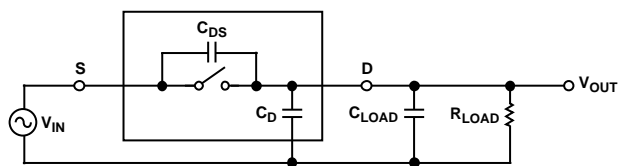
Figure 19. Off Isolation Affected by External Load Resistance and Capacitance
