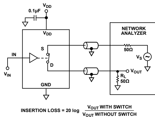
Figure 19. Bandwidth
