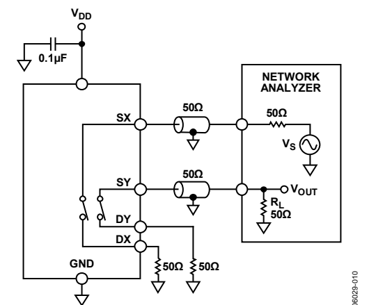
Figure 27. Channel-to-Channel Crosstalk
