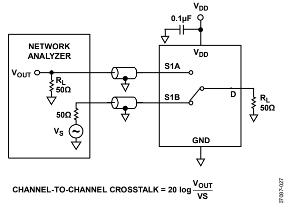
Figure 24. Channel-to-Channel Crosstalk (S1A to S1B/S2A to S2B)
