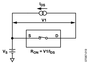
Figure 16. On Resistance
