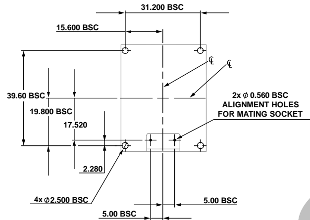
Figure 23. Suggested Mounting Hole Locations, Connector Down
