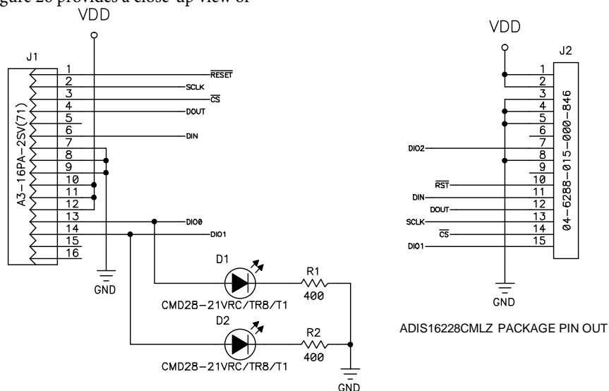
Figure 27. Electrical Schematic
