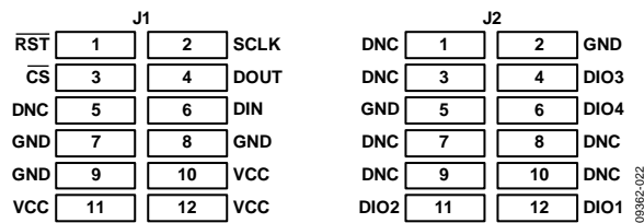
Figure 24. J1/J2 Pin Assignments for Interface PCB
