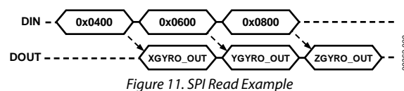
Figure 11. SPI Read Example
