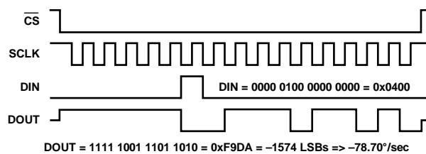
Figure 12. Example SPI Read, Second 16-Bit Sequence
