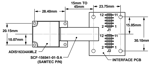
Figure 23. Physical Diagram for Mounting the ADIS16334/PCBZ
